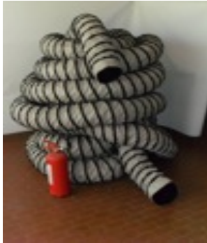
Suction hose for avio fuel vapours id 200mm x 50 meters long single length (supplied to Airlines company)
